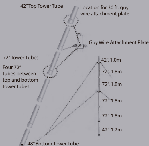
WINDFORCE™ -TOWER – ISLANDERS Complete 8.8-meters Tower KIT for Wind Generators
