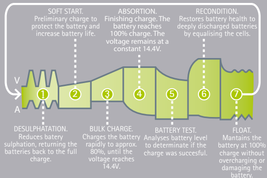
7 Stage Automatic Digital Charger (example for 12V models)
